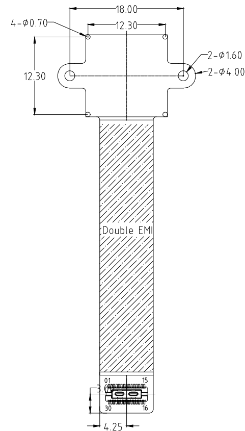
BOTTEM VIEW
